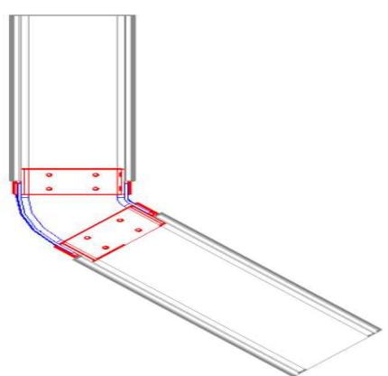
Elbow 45° Horizontal
