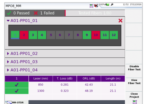
Figure 3. OTDR Optical Switch Interface
