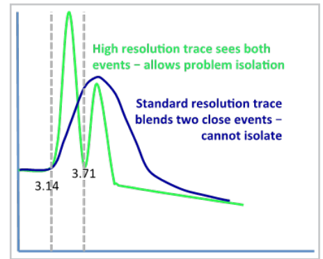
Figure 5. Resolution comparison standard-res OTDR to EVO-A
