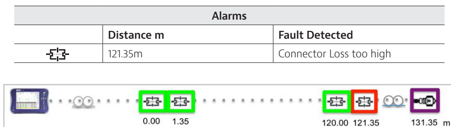
Figure 9. Hi-res link test with MPO cassettes as viewed in Enterprise SLM
